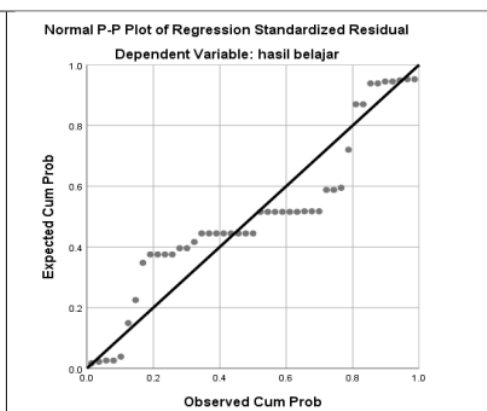
Figure 2. Spread PP – Data Normality Test Plot
