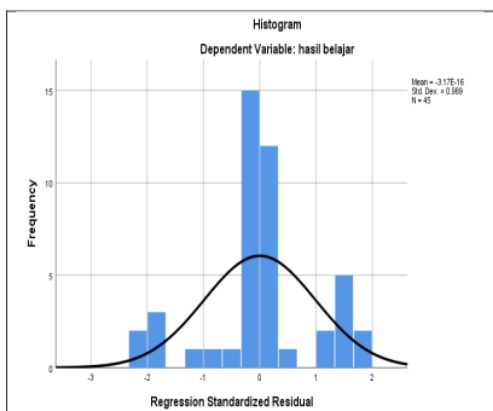
Figure 1. Histogram of Data Normality Test Results
